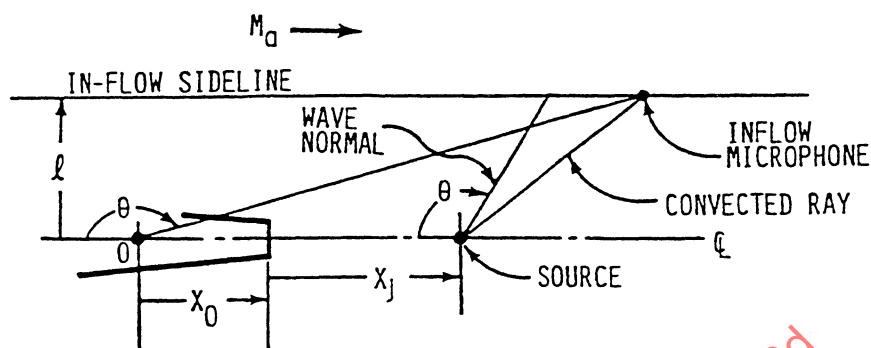
FIGURE 7.2a - In-Flow Coordinates
