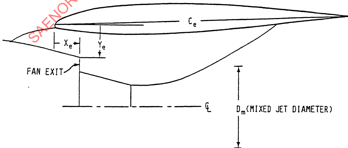
FIGURE 7.3 - Schematic of Installation Parameters
