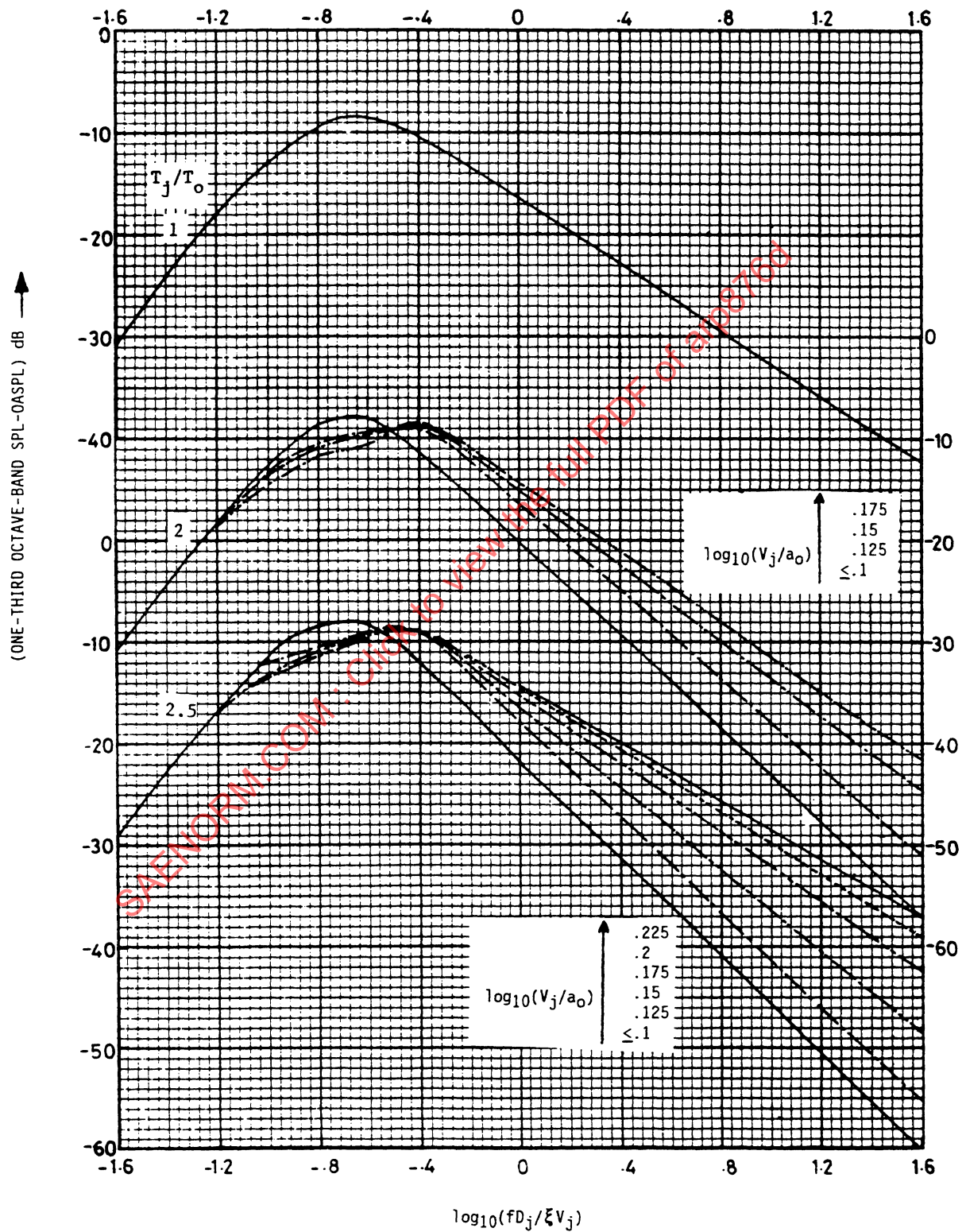
FIGURE 5.11 - One-third Octave-band Normalized Spectra \theta_i = 160^\circ
