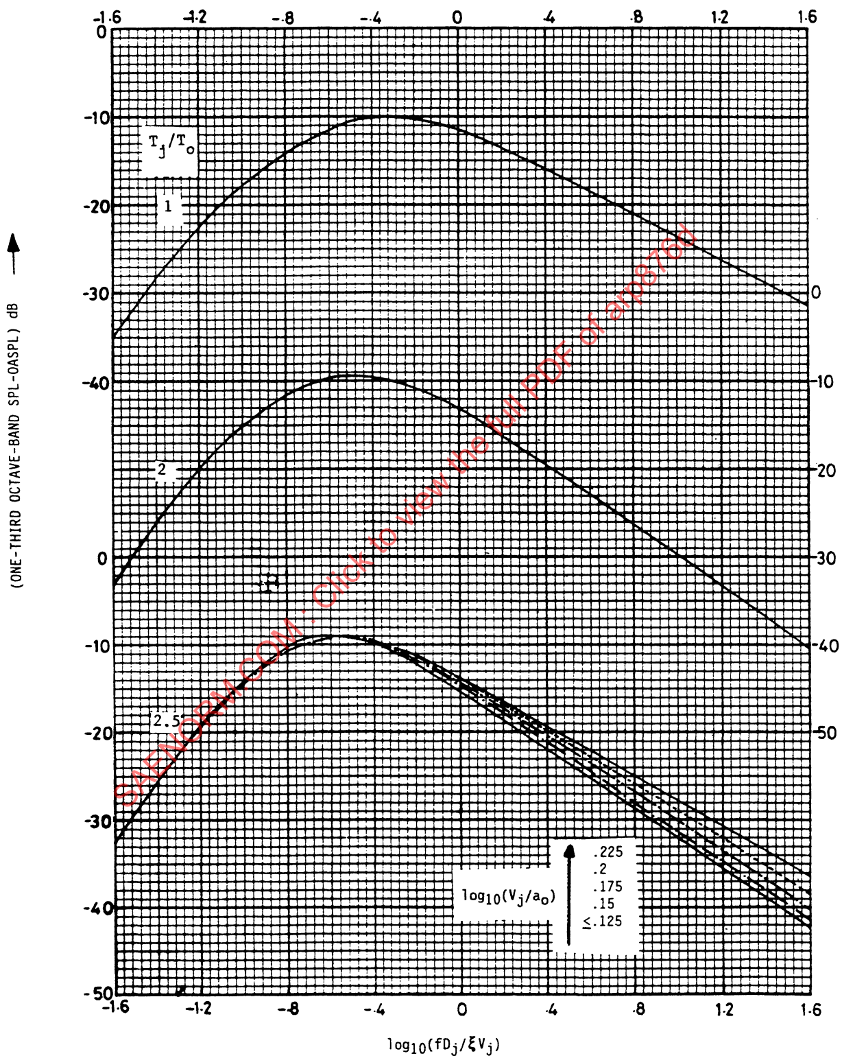
FIGURE 5.9 - One-third Octave-band Normalized Spectra \theta_1 = 140^\circ
