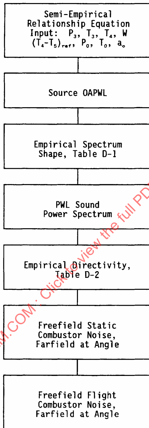
FIGURE 19 - Flow Chart for Combustor Noise Prediction
