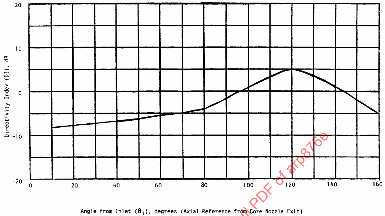
FIGURE 21 - Fairfield Directivity for Combustor Noise
