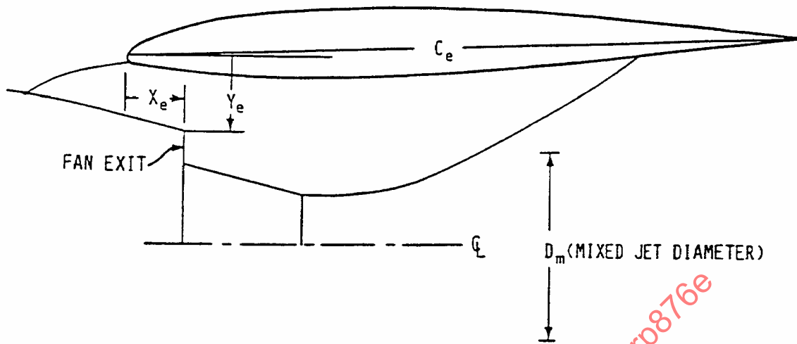
FIGURE 18 - Schematic of Installation Parameters
