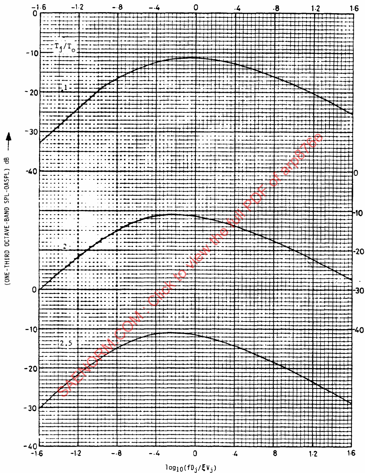
FIGURE 5 - One-third Octave-band Normalized Spectra \theta_i \leq 90^\circ
