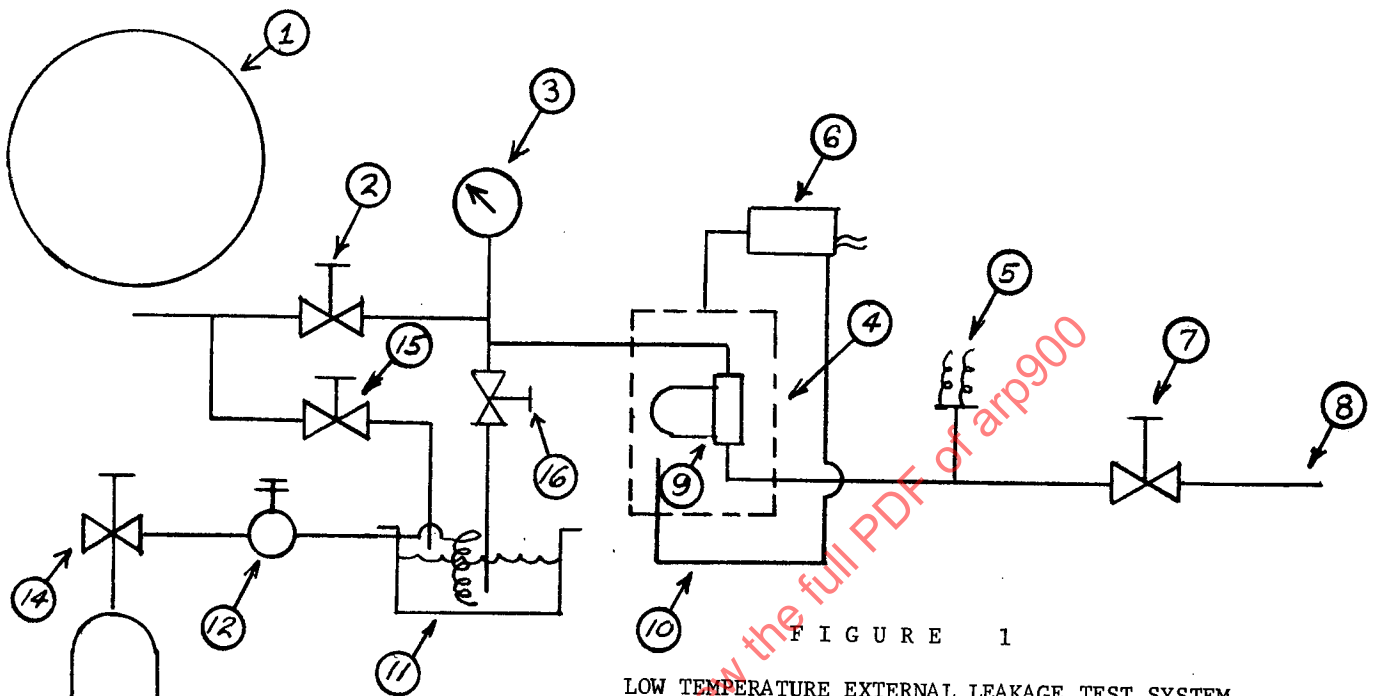
LOW TEMPERATURE EXTERNAL LEAKAGE TEST SYSTEM
