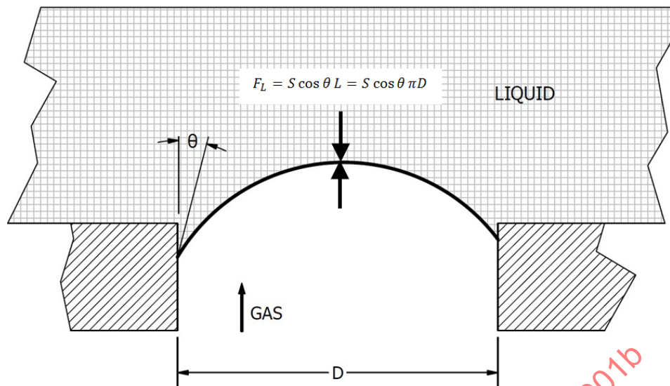
Figure A1 - Circular capillary model
