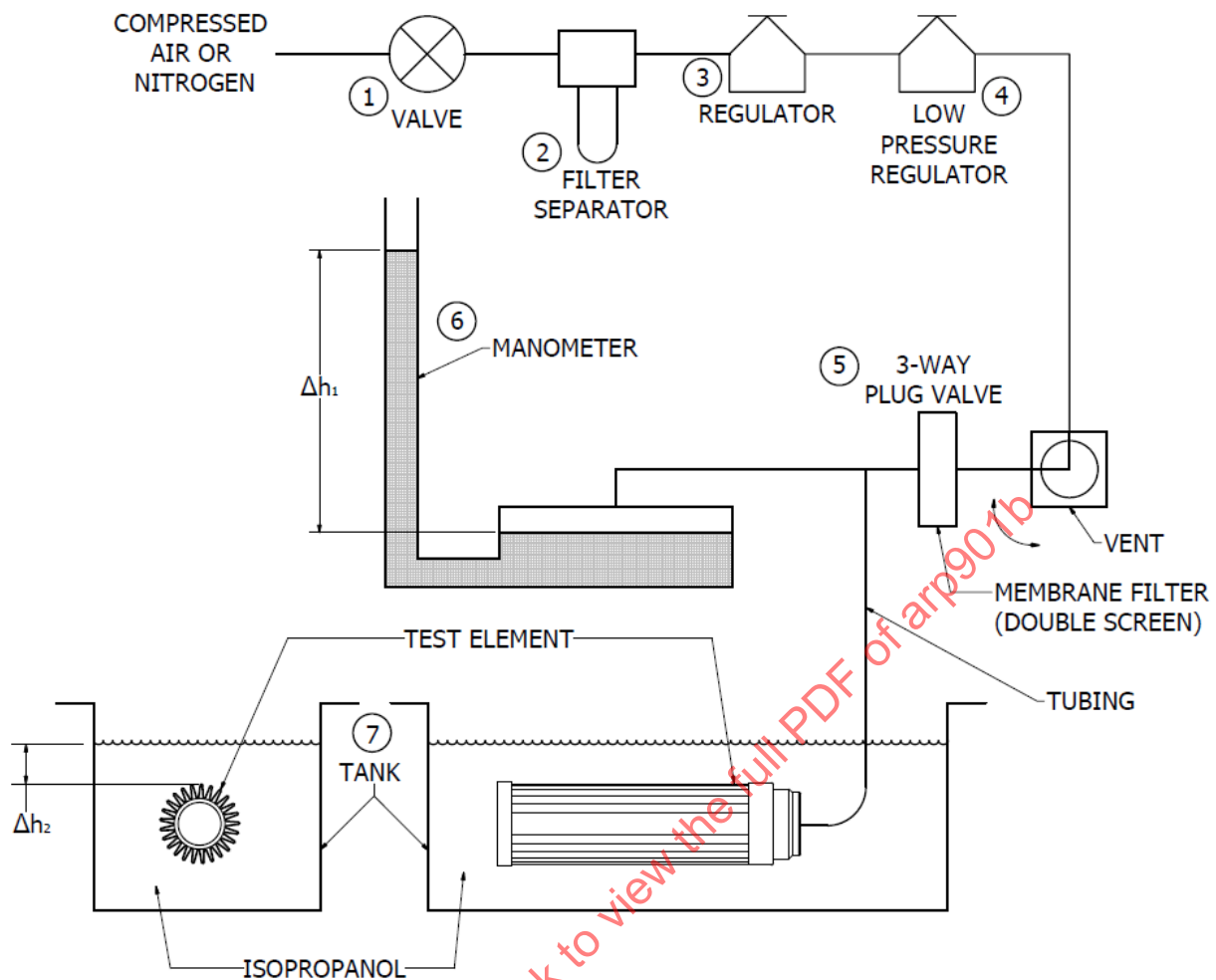
Figure 1 - Bubble-point test apparatus
