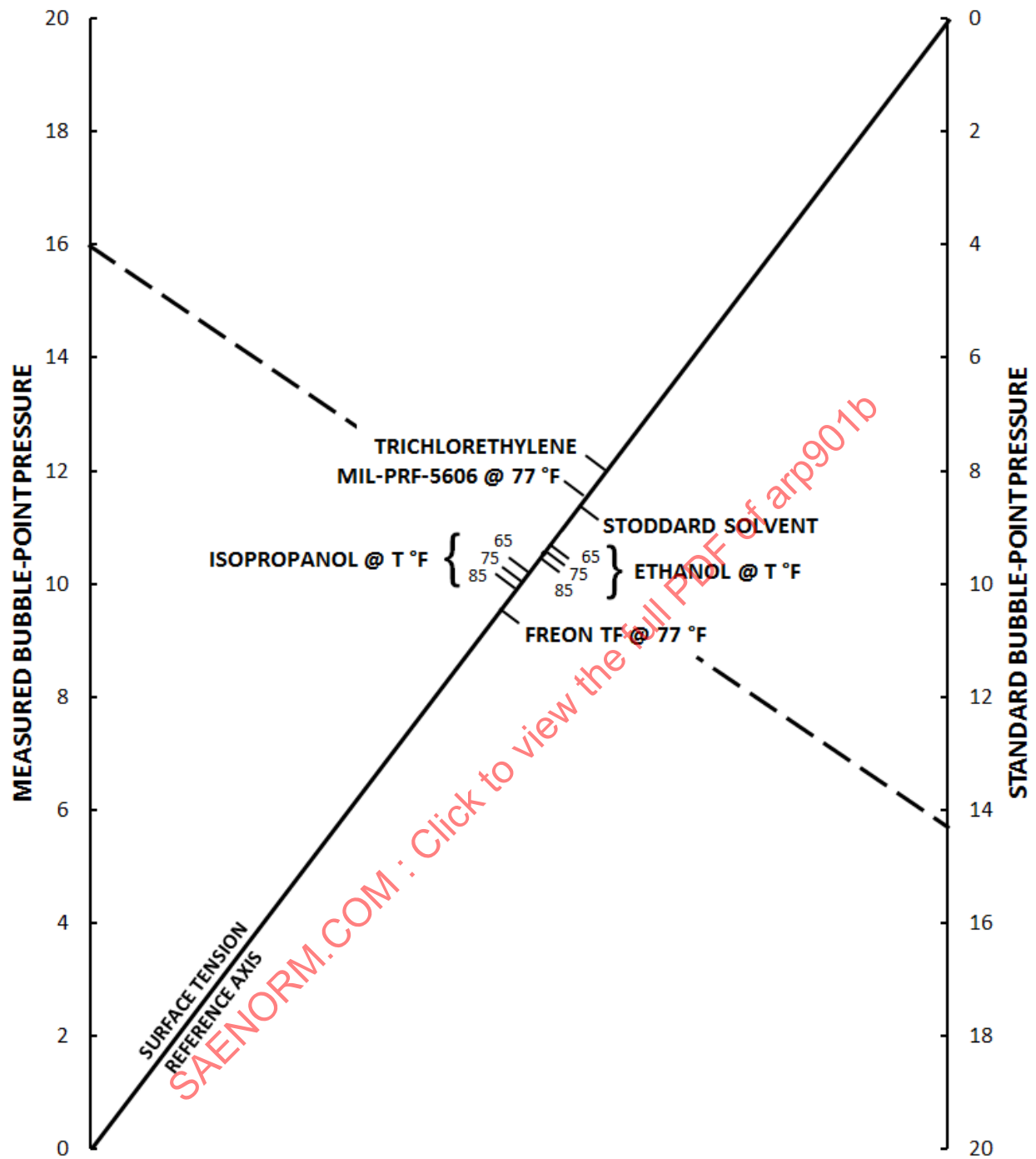
Figure 4A - Bubble-point correction nomograph, degrees fahrenheit
