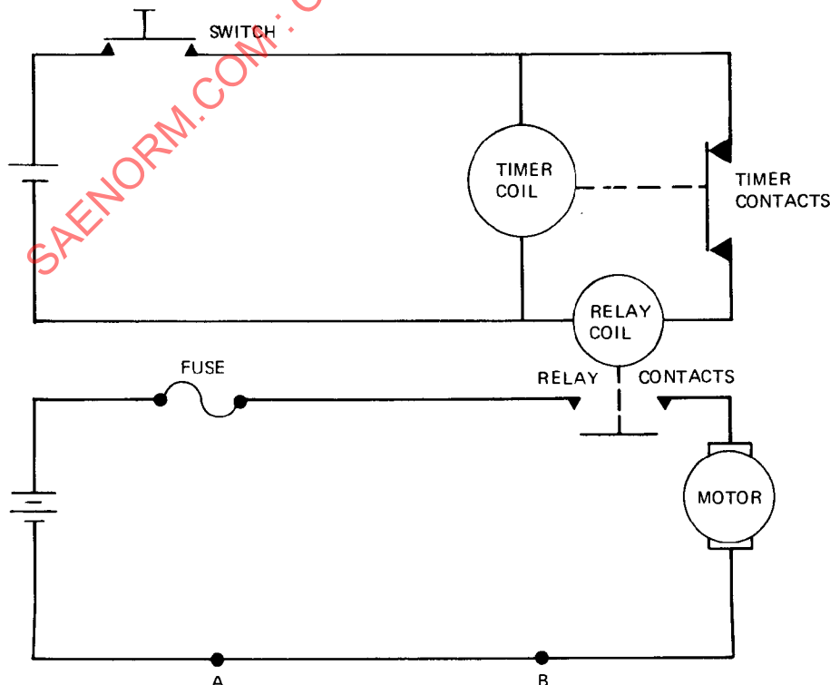
FIGURE 21 SAMPLE SYSTEM
