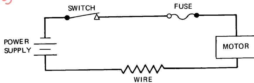
FIGURE 17 SAMPLE SYSTEM
