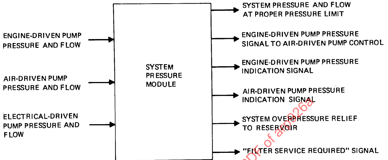
FIGURE 6 COMPONENT FUNCTIONAL BLOCK DIAGRAM
