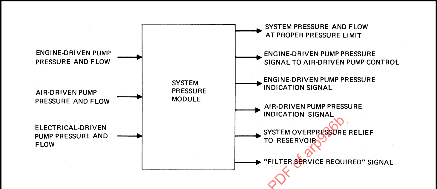
FIGURE 6 - Component Functional Block Diagram
