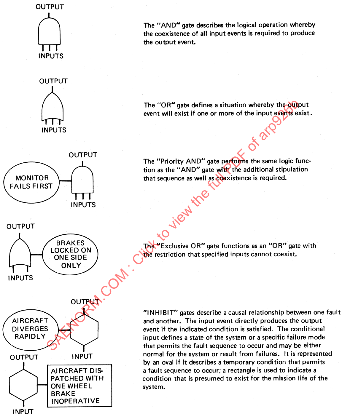
FIGURE 13 - Logic Operations (Gates)
