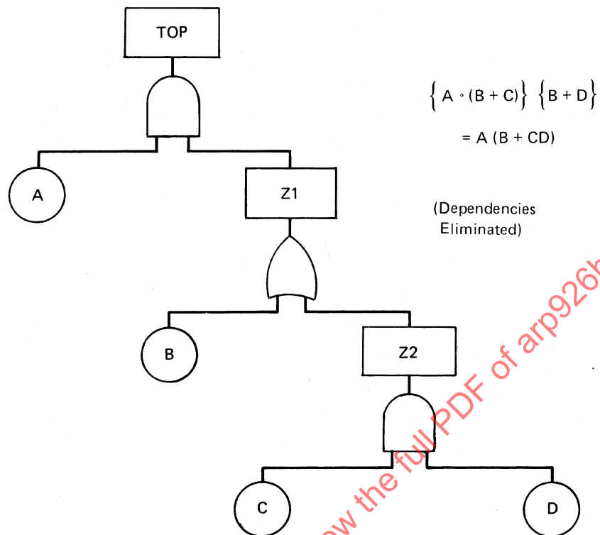
FIGURE 20 - Boolean Equivalent of Sample Fault Tree Shown in Figure 19
