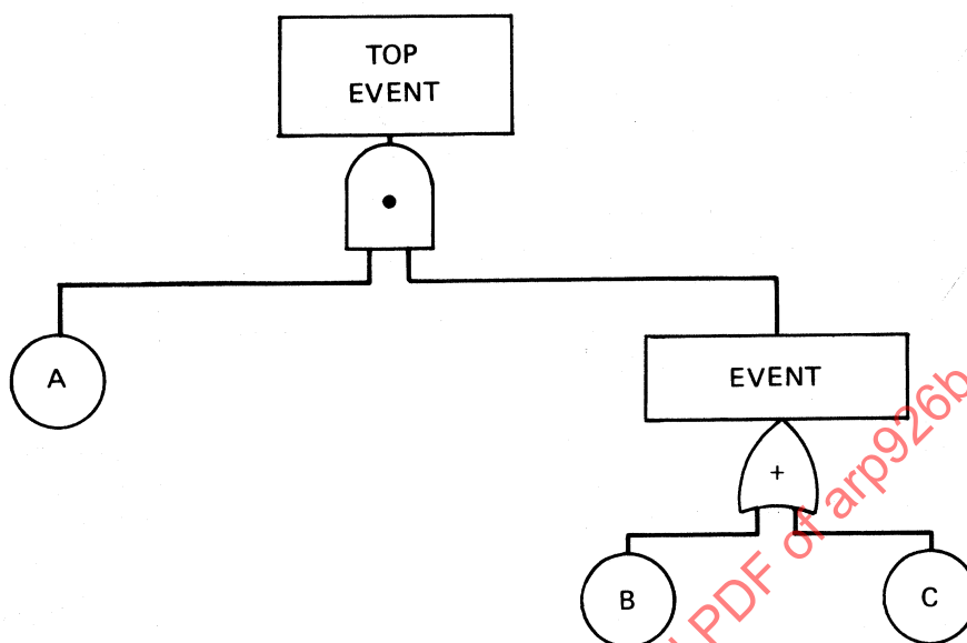
FIGURE 16 - Fault Tree
