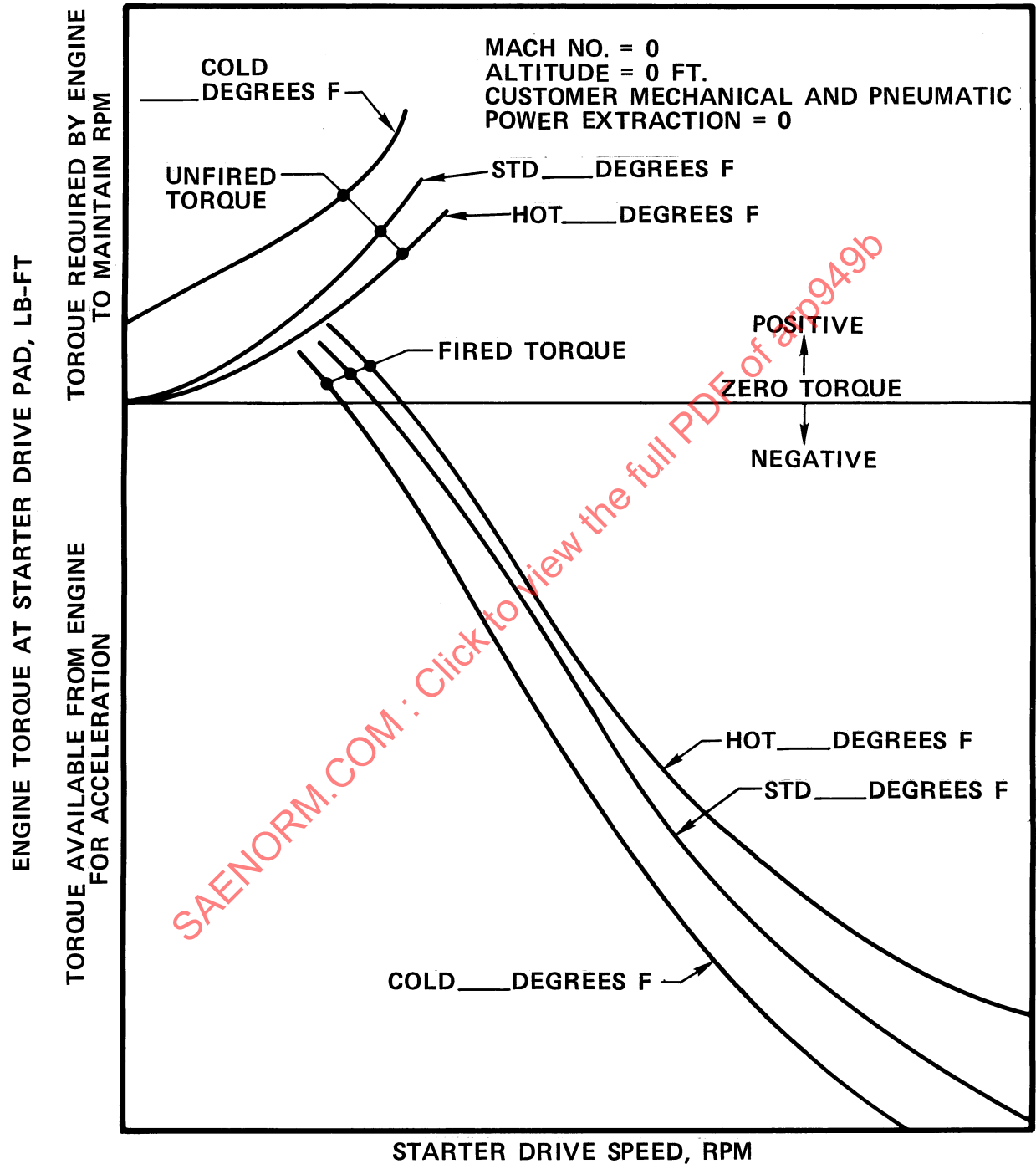
FIGURE 1 - Fired and Unfired Engine Torque Characteristics and Effect of Ambient Temperature
