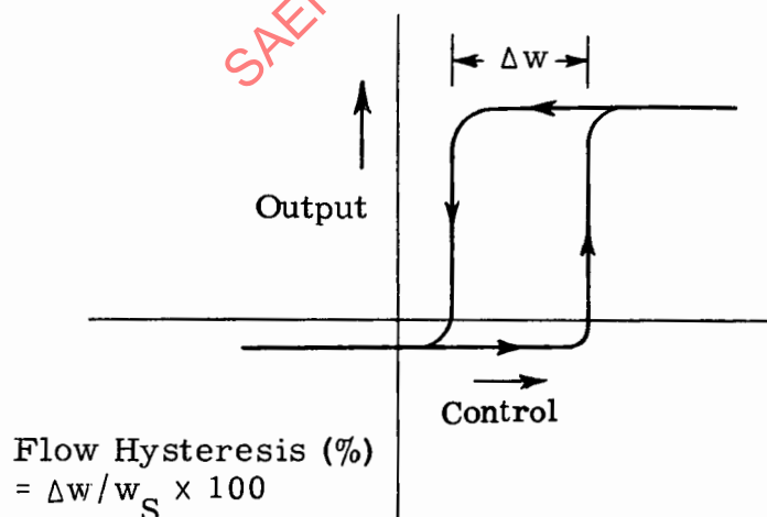
Figure 4.2 Hysteresis Definition
