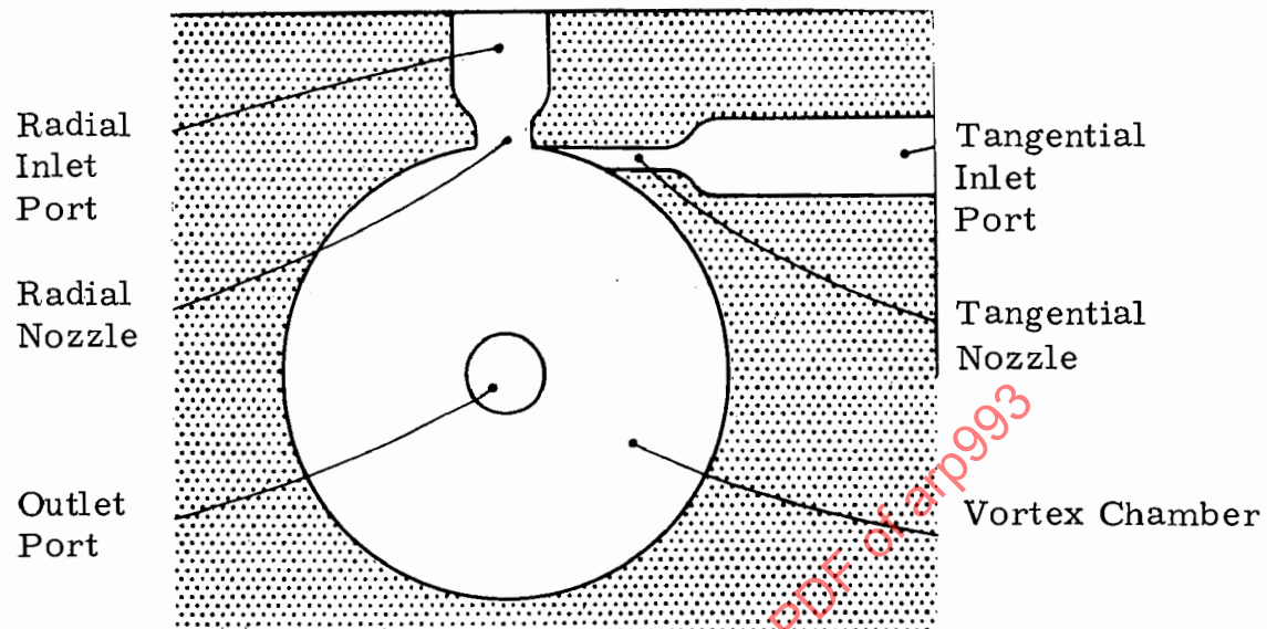
Figure 2.3 Vortex Amplifier
