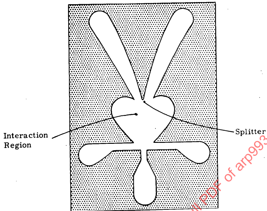
Figure 2.1(b) Closed Jet Interaction Amplifier.
