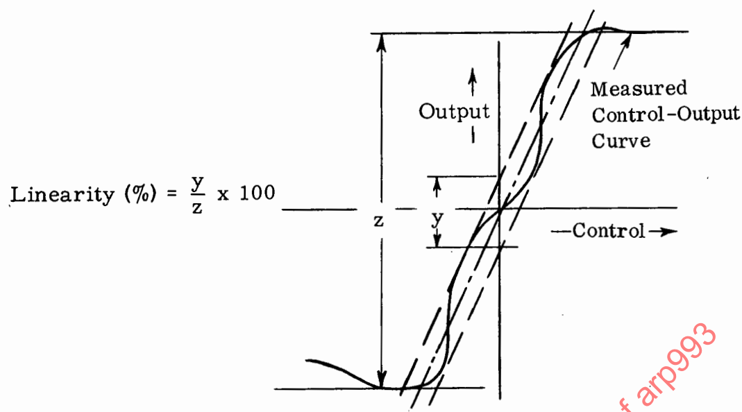
Figure 4.5 Linearity Definition
