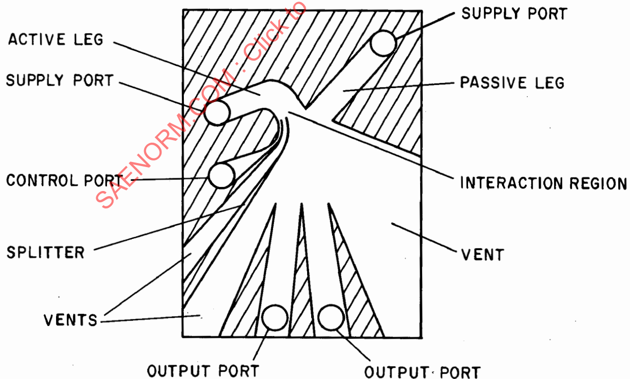
Figure 2.4 Boundary Layer Control Amplifier (Vents Optional)
