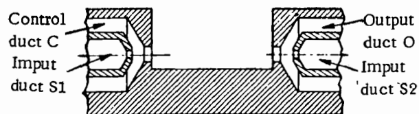
Direct Impact Modulator
