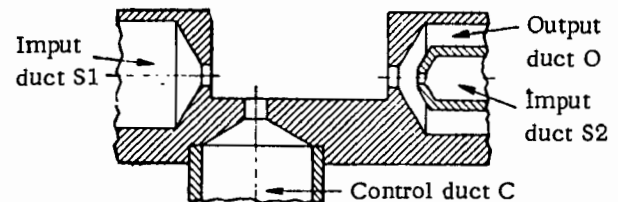
Transverse Impact Modulator
