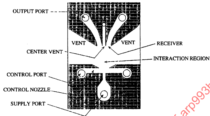
FIGURE 1 - Jet Interaction Amplifier
