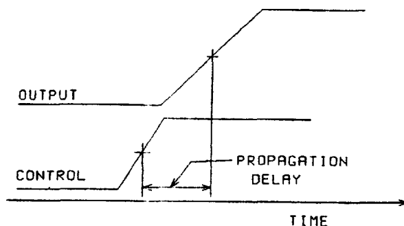
FIGURE 14 - Propagation Delay
