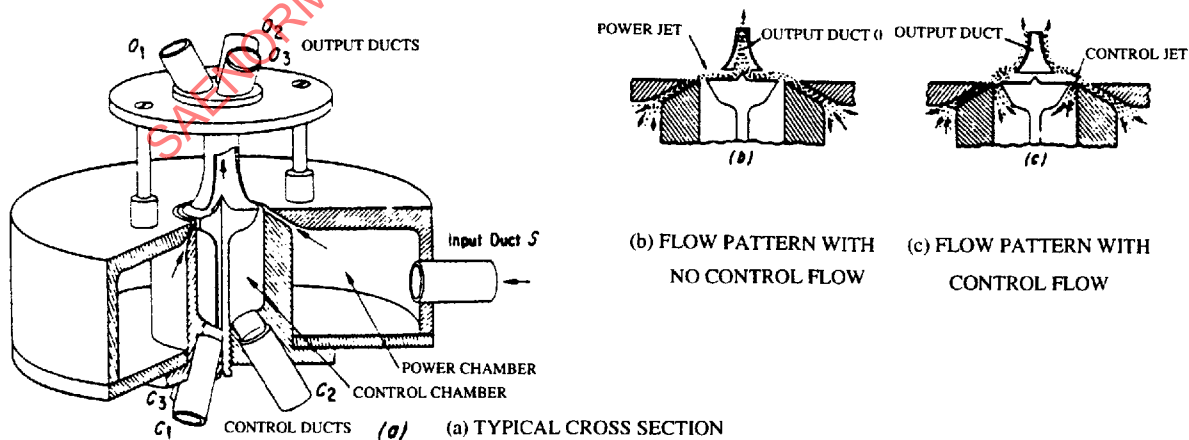
FIGURE 5 - Focused - Jet Amplifier
