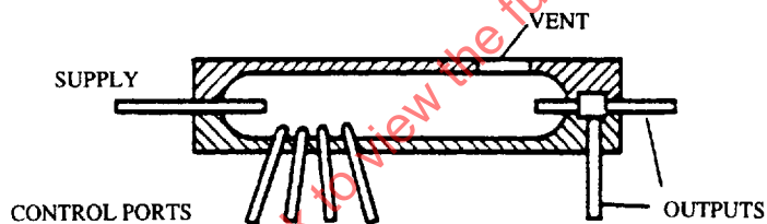
FIGURE 4 - Turbulence Amplifier
