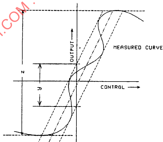
FIGURE 19 - Linearity
