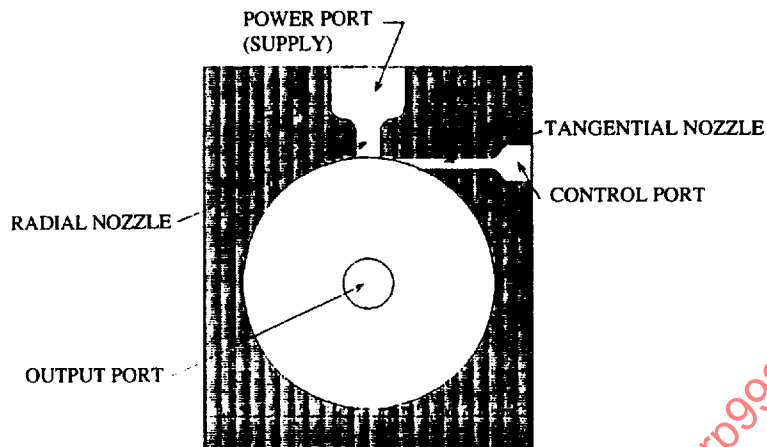
FIGURE 3 - Vortex Amplifier
