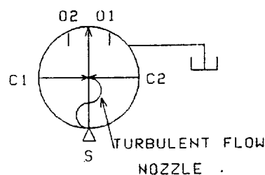
DIFFERENTIAL JET INTERACTION ANALOG AMPLIFIER
