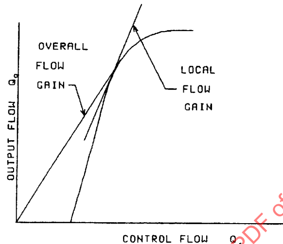
FIGURE 17 - Flow Gain
