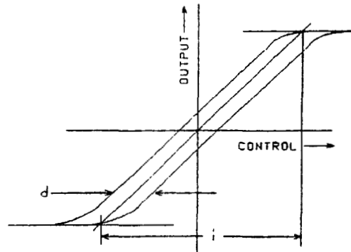
FIGURE 20 - Hysteresis in Proportional Elements
