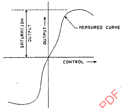
FIGURE 18 - Saturation
