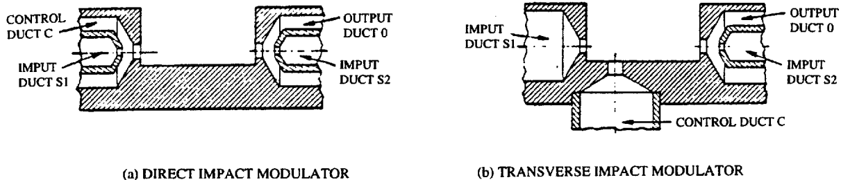
FIGURE 6 - Impact Modulators
