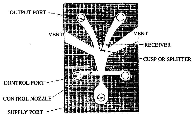
FIGURE 2 - Wall Attachment Amplifier
