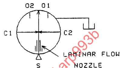
DIFFERENTIAL JET INTERACTION ANALOG AMPLIFIER
