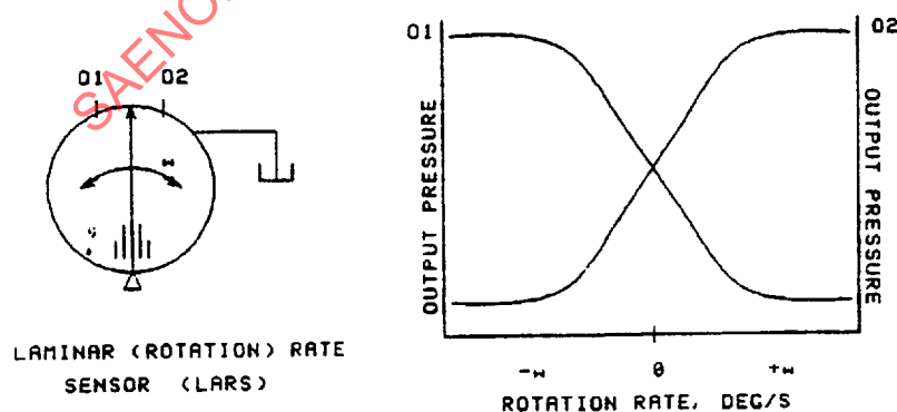
FIGURE 11 - Analog Fluidic Devices
