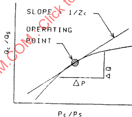
FIGURE 21 - Control Impedance
