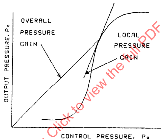
FIGURE 16 - Pressure Gain
