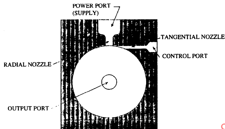
FIGURE 3 - Vortex Amplifier
