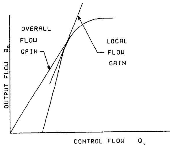
FIGURE 17 - Flow Gain
