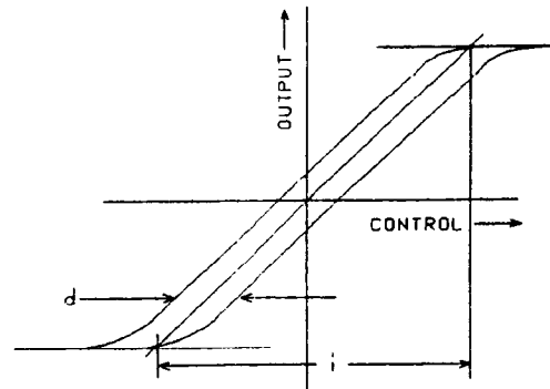
FIGURE 20 - Hysteresis in Proportional Elements
