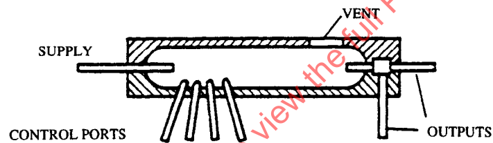
FIGURE 4 - Turbulence Amplifier
