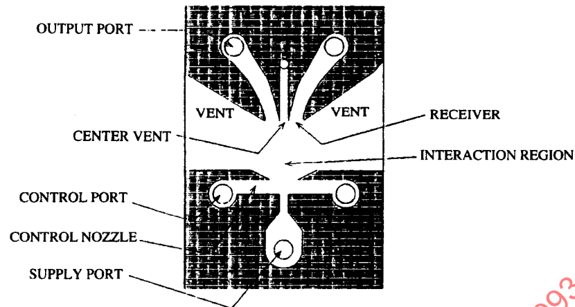
FIGURE 1 - Jet Interaction Amplifier
