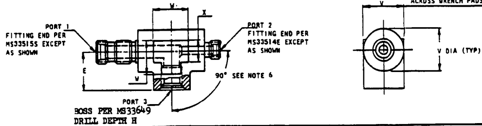
REDUCER COMBINATIONS
