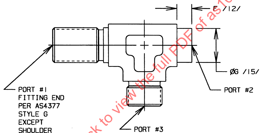
FIGURE 4 - FITTING, TEE, BULKHEAD END NOT FOR USE IN PORT INSTALLATION, PORT #2 SHOWN AS REDUCER, SAME AS FIGURE 1 EXCEPT AS SHOWN
