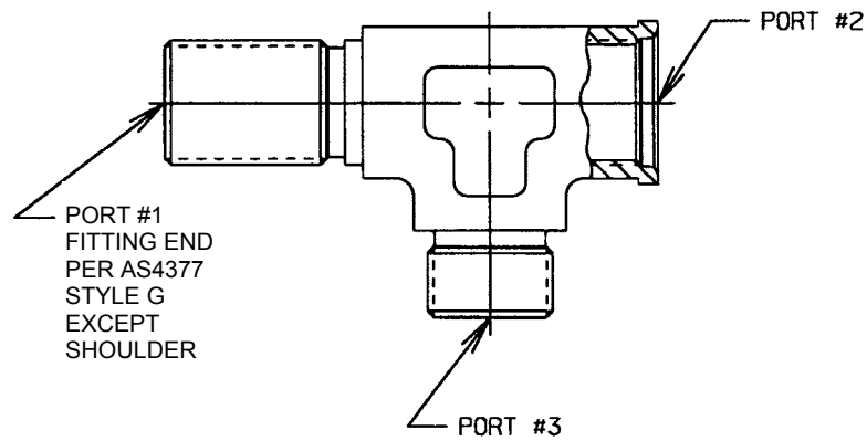
FIGURE 3 - FITTING, TEE, BULKHEAD END NOT FOR USE IN PORT INSTALLATION, PORT #2 SHOWN AS NON-REDUCER, SAME AS FIGURE 1 EXCEPT AS SHOWN
