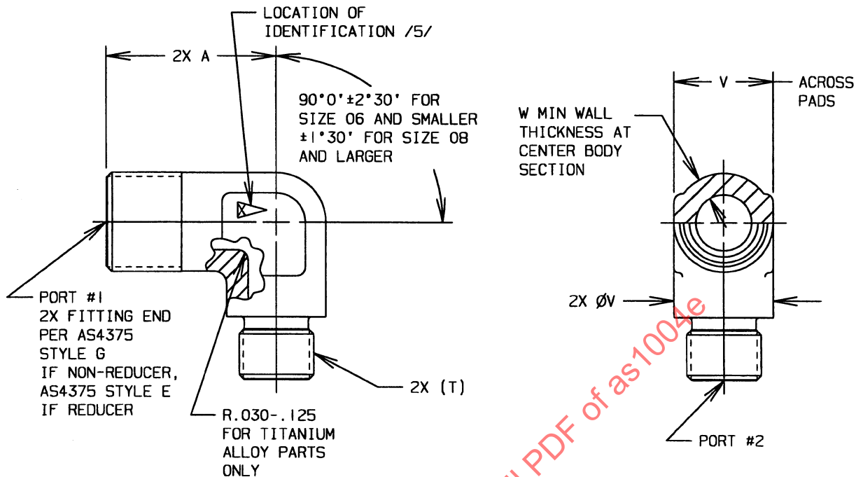
FIGURE 1 - FITTING, ELBOW, 90°
