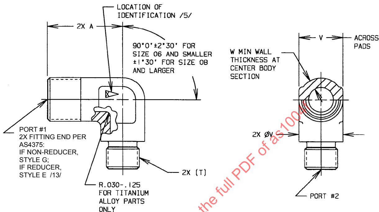
FIGURE 1 - FITTING, ELBOW, 90°, PORT #2 SHOWN AS REDUCER
