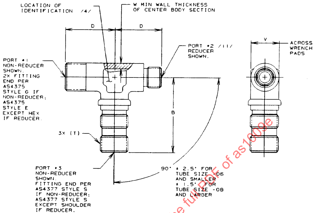
FIGURE 1 - TEE, BULKHEAD ON SIDE
