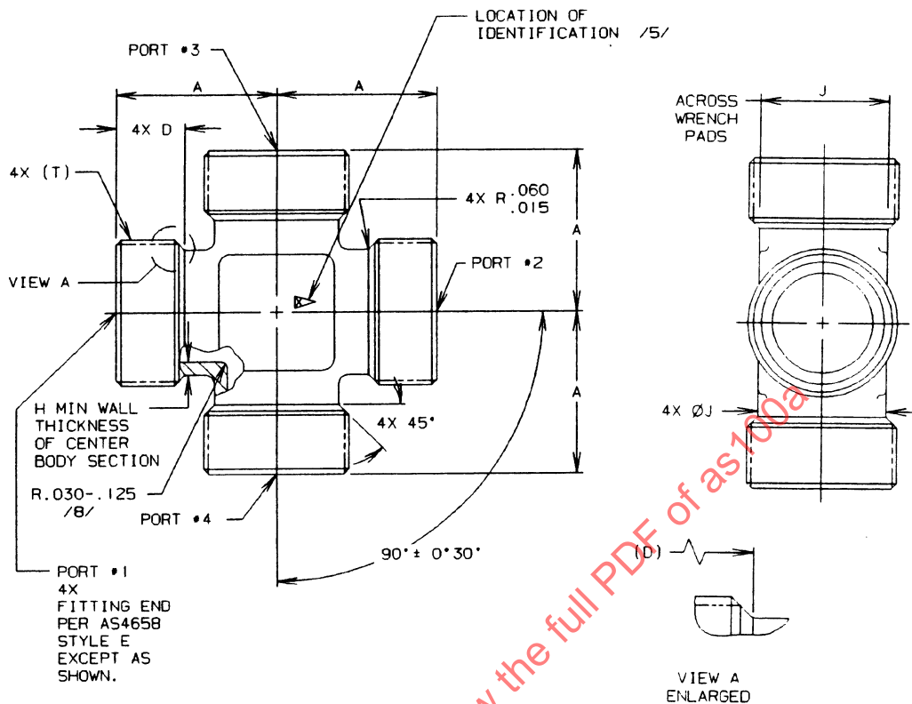
FIGURE 1 - FITTING, CROSS
