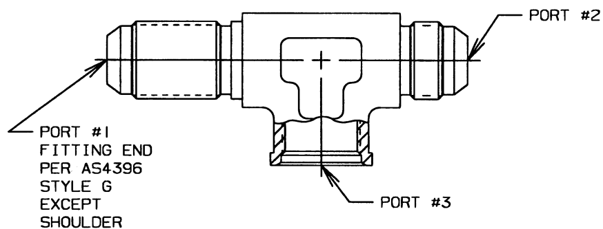
FIGURE 3 - FITTING, TEE, BULKHEAD END NOT FOR USE IN PORT PORT #3 SHOWN AS NON-REDUCER SAME AS FIGURE 1 EXCEPT AS SHOWN /23/
