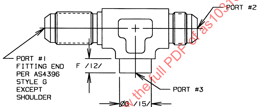
FIGURE 4 - FITTING, TEE, BULKHEAD END NOT FOR USE IN PORT PORT #3 SHOWN AS REDUCER SAME AS FIGURE 1 EXCEPT AS SHOWN /23/
