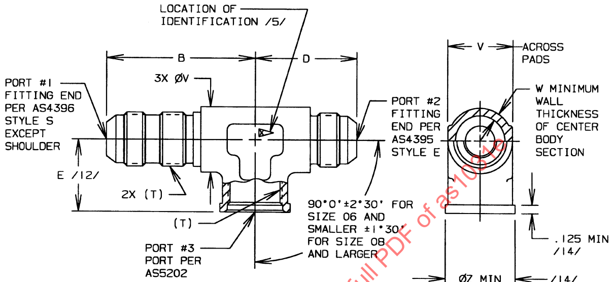
FIGURE 1 - FITTING, TEE, BULKHEAD END FOR OPTIONAL USE IN PORT PORT #3 SHOWN AS NON-REDUCER
