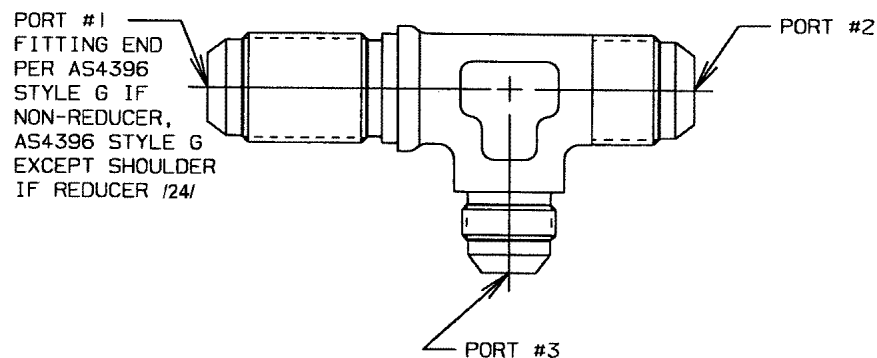
FIGURE 3 - FITTING, TEE, BULKHEAD END NOT FOR USE IN PORT PORT #3 SHOWN AS REDUCER SAME AS FIGURE 1 EXCEPT AS SHOWN, /21/ BULKHEAD END, NOT FOR USE IN PORT
