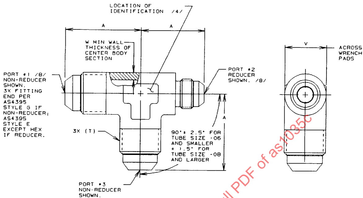
FIGURE 1 - TEE, FLARED
