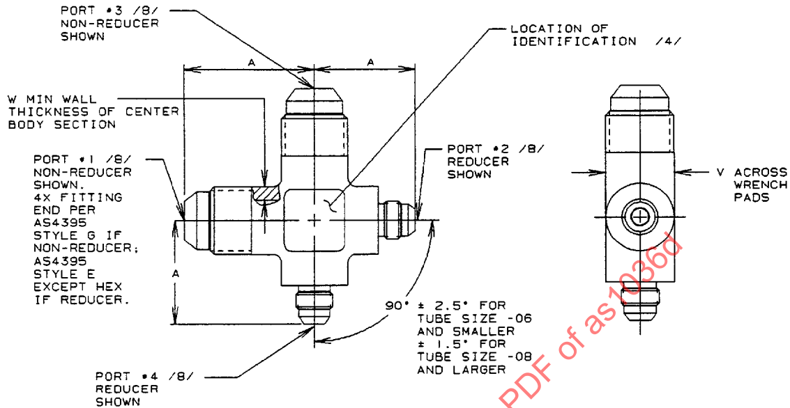
FIGURE 1 - CROSS, FLARED
