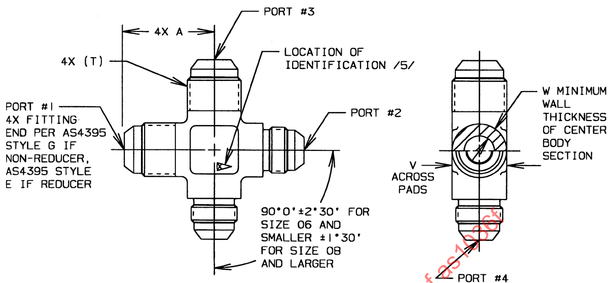
FIGURE 1 - CROSS, FLARED
