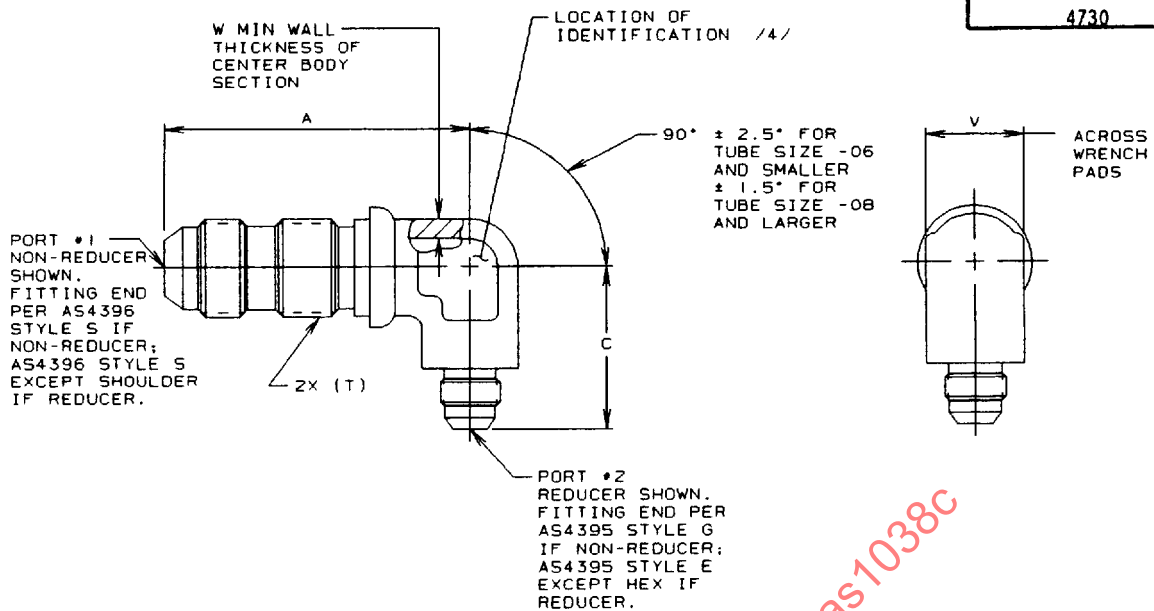
FIGURE 1 - ELBOW, 90°, BULKHEAD
