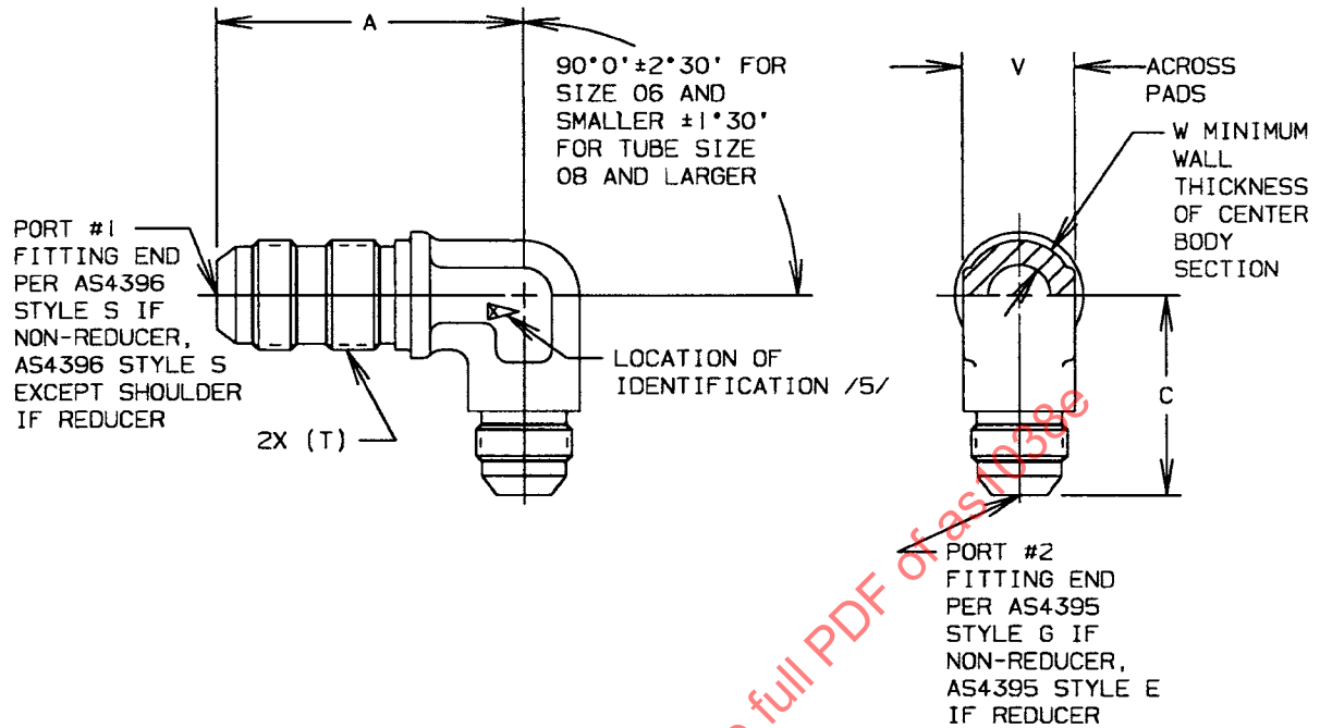
FIGURE 1 - FITTING, ELBOW, 90°, BULKHEAD END FOR OPTIONAL USE IN PORT PORT #2 SHOWN AS REDUCER
