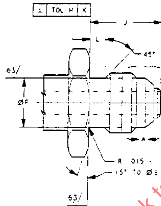
FIGURE 2 - FITTING END, SEAL RING, STYLE E
