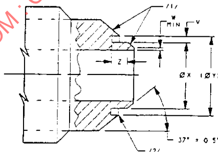
FIGURE 3 - ENLARGED VIEW A FROM FIGURES 1 AND 2
