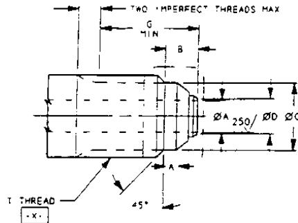
FIGURE 1 - FITTING END, SEAL RING, STYLE G
