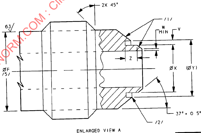
FIGURE 2 - FITTING END, STYLE E, BULKHEAD FLARED TUBE, FOR SEAL RING
