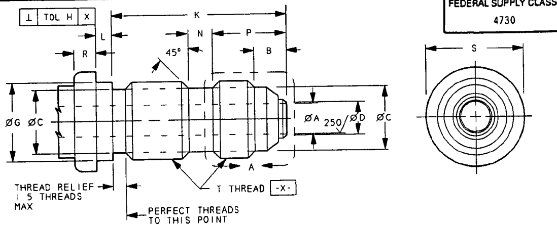
FIGURE 1 - FITTING END, STYLE S, BULKHEAD FLARED TUBE, FOR SEAL RING
