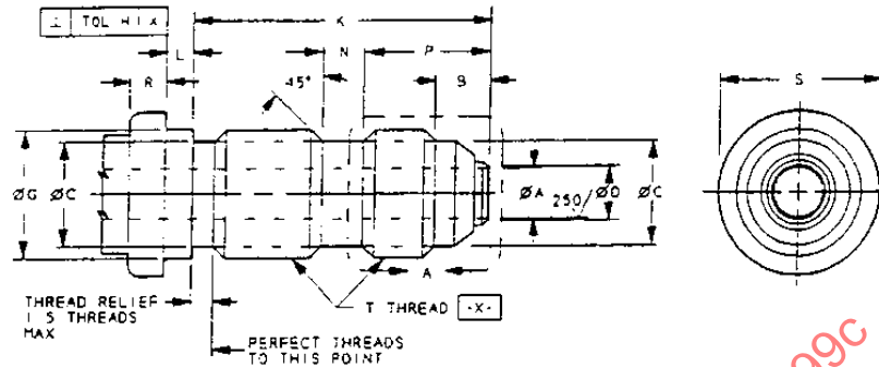
FIGURE 1 - FITTING END, STYLE S, BULKHEAD FLARED TUBE, FOR SEAL RING
