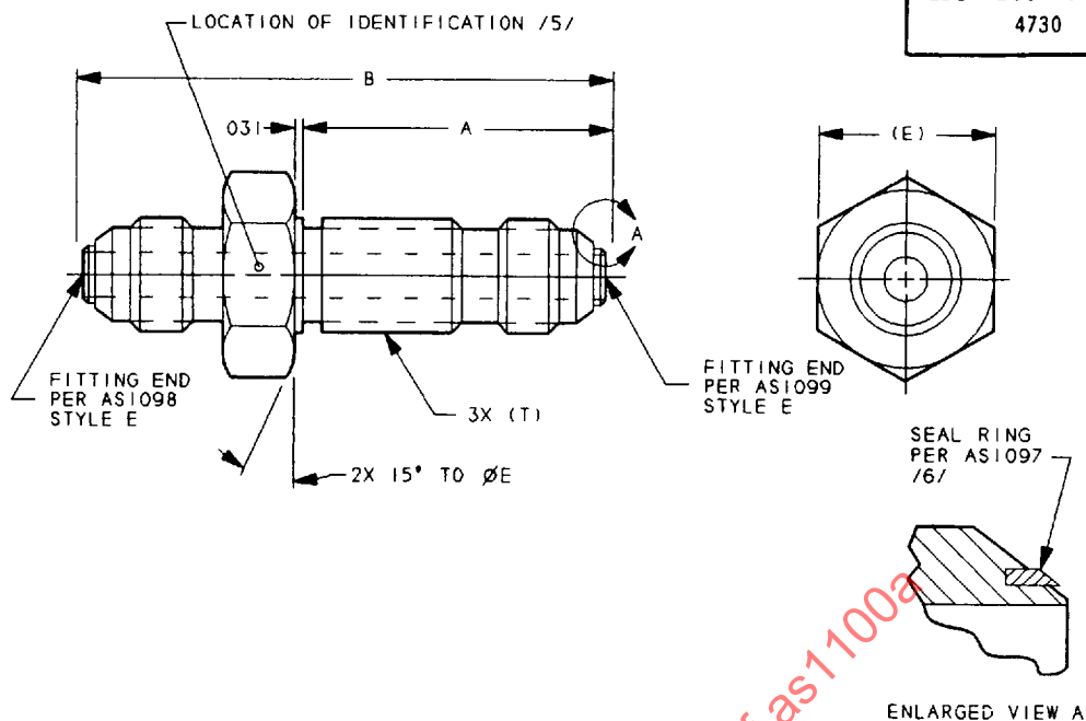
FIGURE 1 - UNION, FLARED TUBE BULKHEAD AND UNIVERSAL
