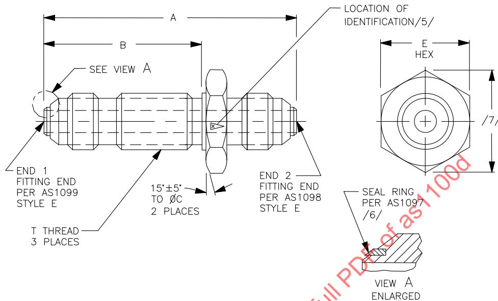
FIGURE 1 - FITTING, UNION, FLARED TUBE, BULKHEAD AND UNIVERSAL
