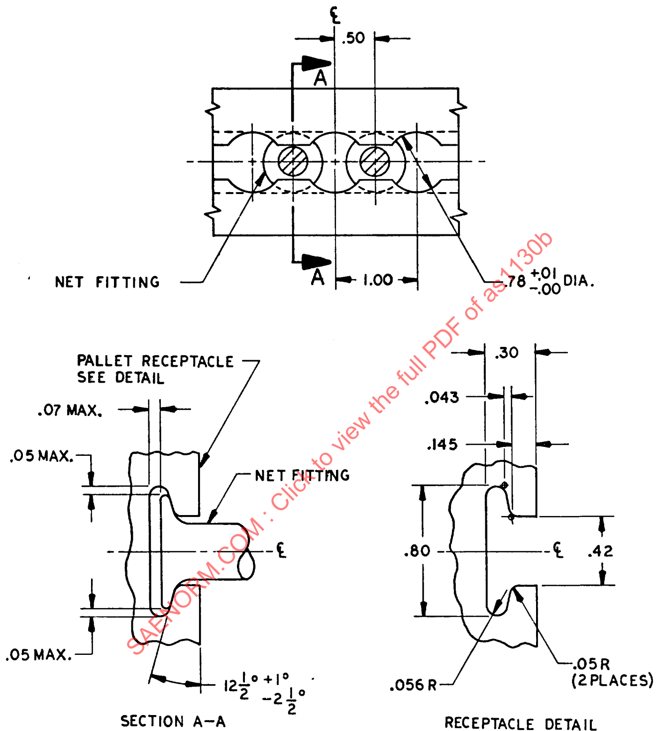
FIGURE 5 CARGO NET TIE-DOWN RECEPTACLE DIMENSION IN INCHES
