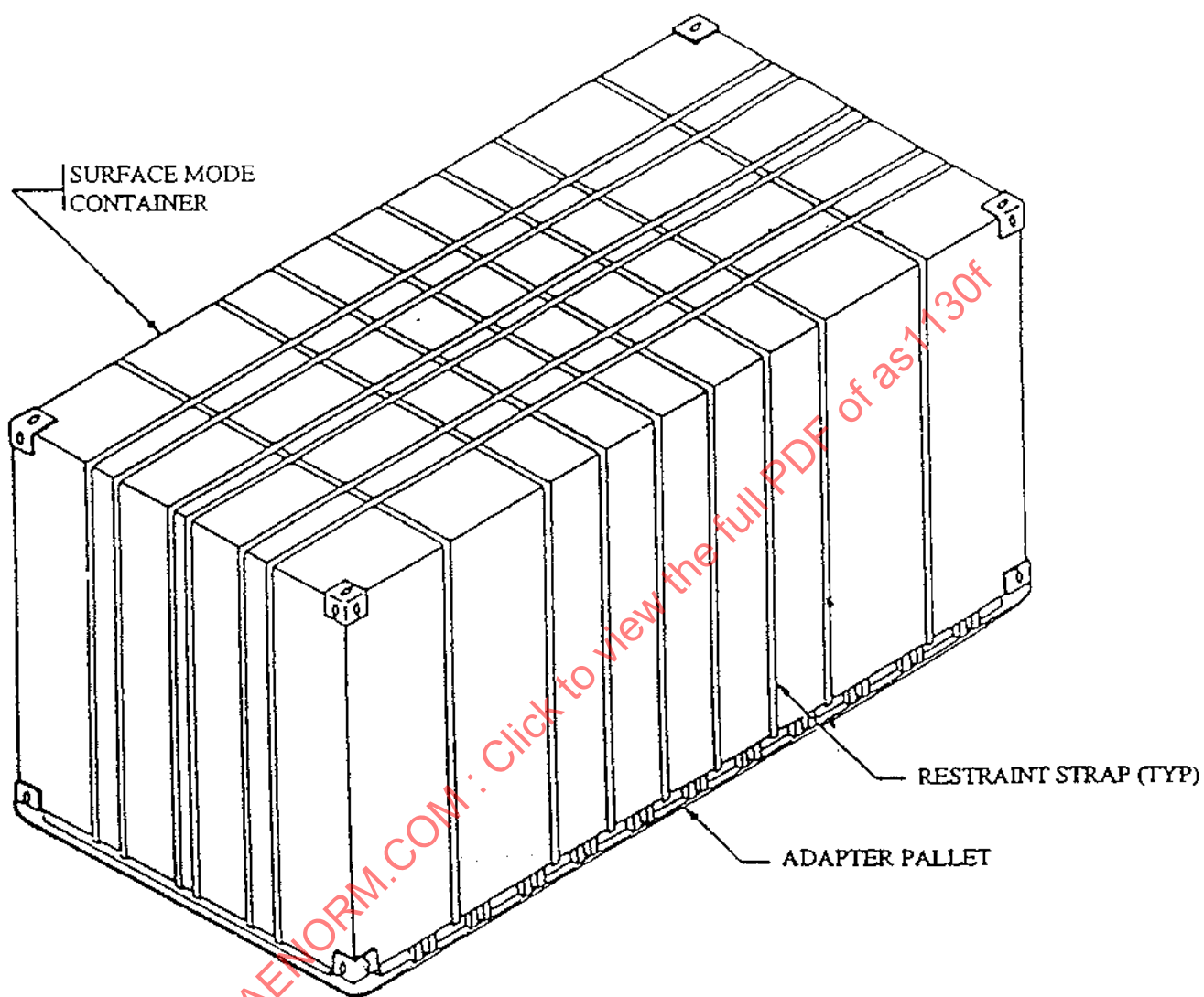
FIGURE 15 - Restraint of 6.06 m (20 ft) Surface Mode Container
