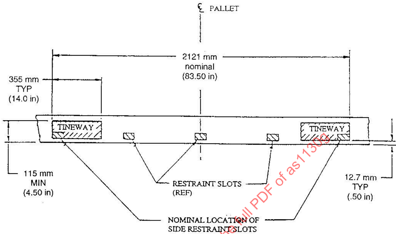
FIGURE 12 - Forklift Tineway Configuration
