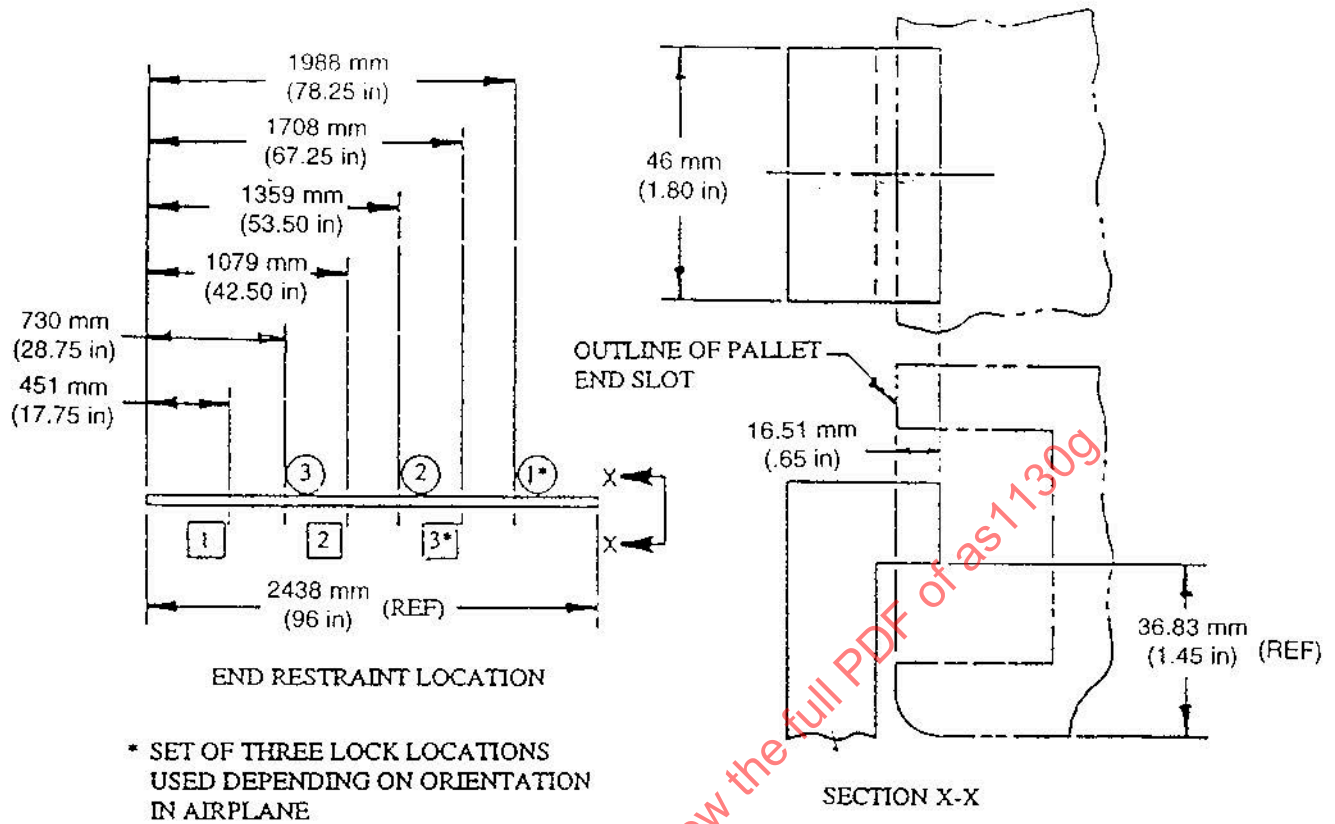
FIGURE 8 - End Restraint Fitting and Locations
