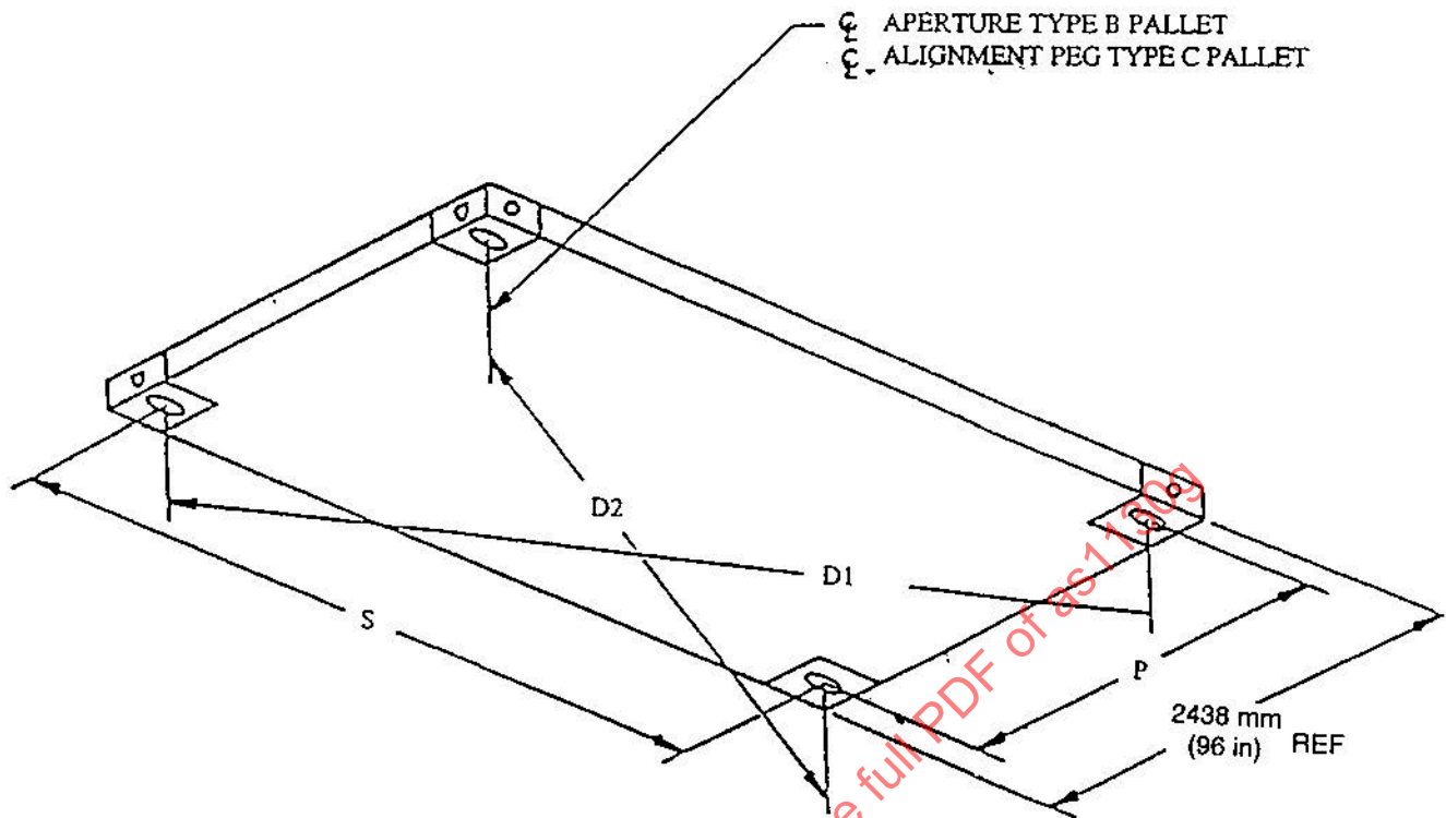
FIGURE 9 - Type B and C Pallet
