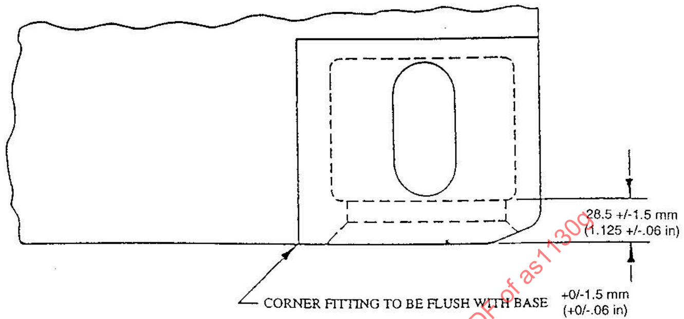
FIGURE 10 - Location of Bottom Corner Fitting Type B Pallet
