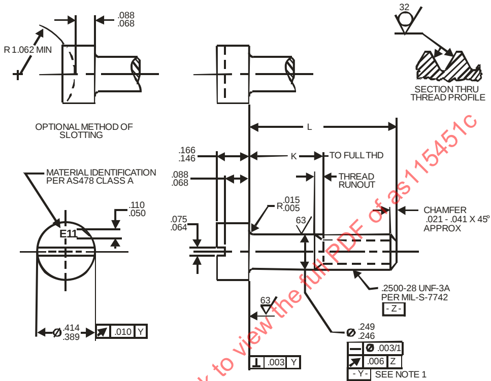
FIGURE 1 – SCREW
