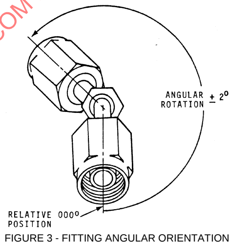
FIGURE 3 - FITTING ANGULAR ORIENTATION
