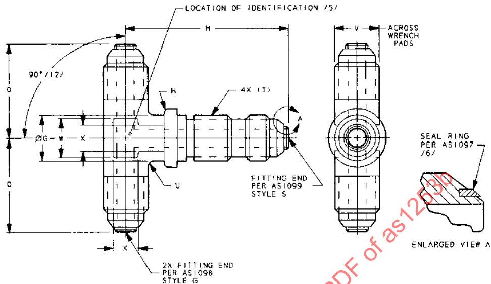
FIGURE 1 - TEE, FLARED TUBE, BULKHEAD UNIVERSAL ON SIDE
