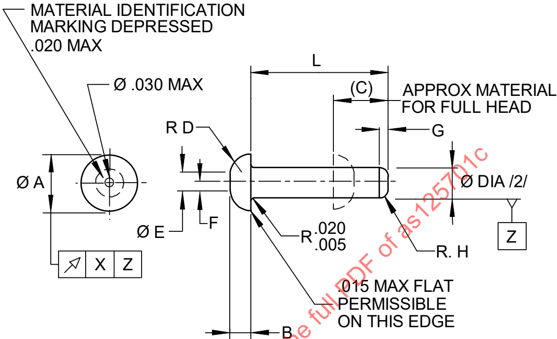
FIGURE 1 – RIVET
