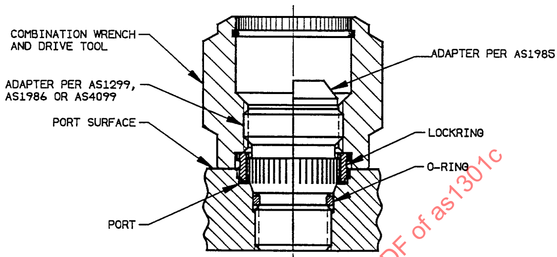
FIGURE 4 - Lockring Installation
