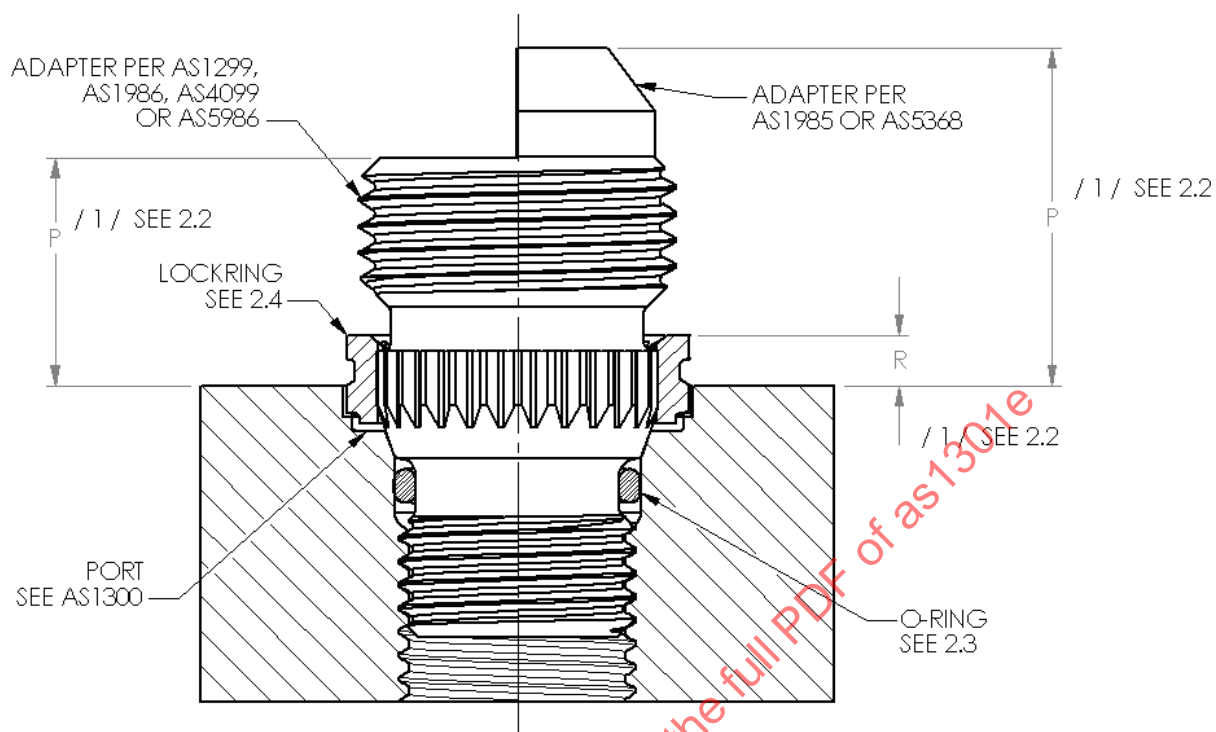
FIGURE 1 - INSTALLED ADAPTER
