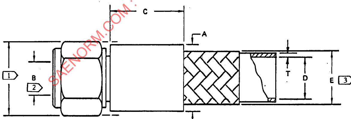
HOSE AND FITTING DIMENSIONS
