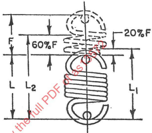
FIGURE 2. Extension springs
