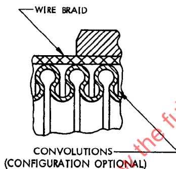
DETAIL I
