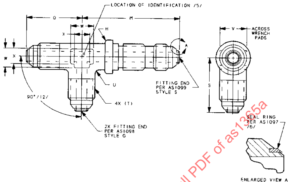
FIGURE 1 - TEE, FLARED TUBE, BULKHEAD UNIVERSAL ON RUN
