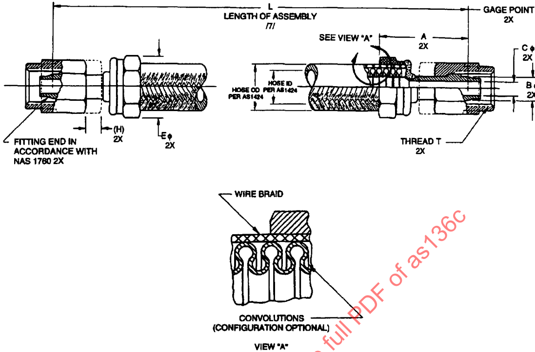
FIGURE 1 - HOSE ASSEMBLY
