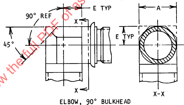
ELBOW, 90° BULKHEAD
