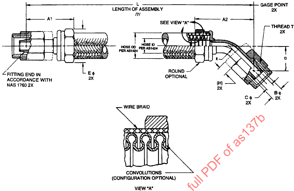
FIGURE 1 - HOSE ASSEMBLY
