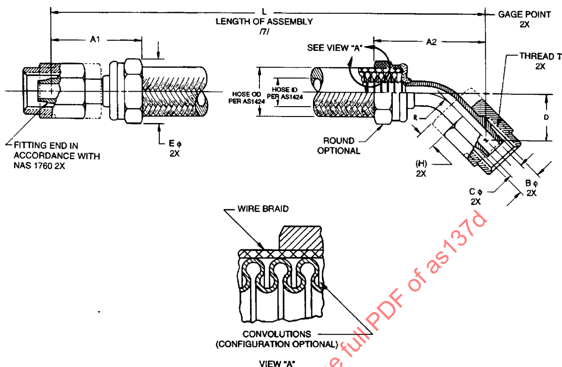
FIGURE 1 - HOSE ASSEMBLY
