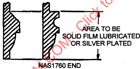
FIGURE 1 - HOSE ASSEMBLY
