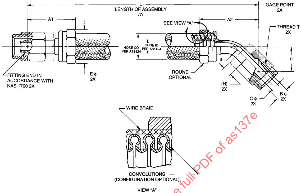
FIGURE 1 - HOSE ASSEMBLY
