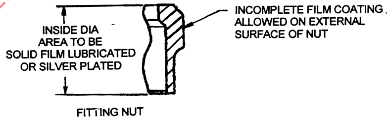
FIGURE 2 - LUBRICANT APPLICATION AREA /14/ /15/
