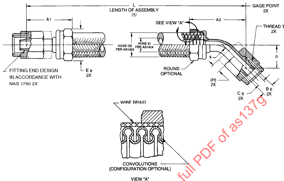
FIGURE 1 - HOSE ASSEMBLY
