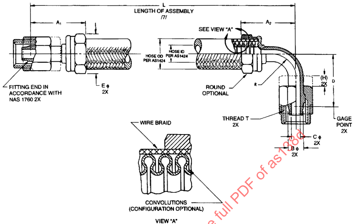
FIGURE 1 - HOSE ASSEMBLY
