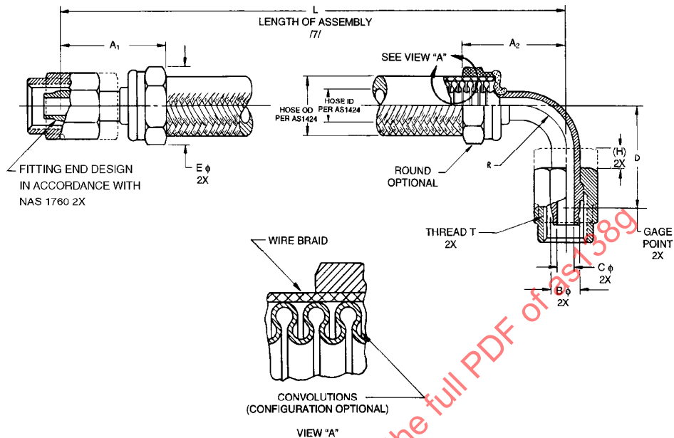
FIGURE 1 - HOSE ASSEMBLY
