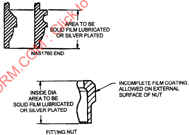
FIGURE 2 - LUBRICANT APPLICATION AREA /14/ /15/
